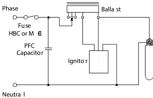
Typical impulser ignitor circuit
