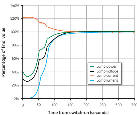
Typical warm-up characteristics for CMH TD 35W
