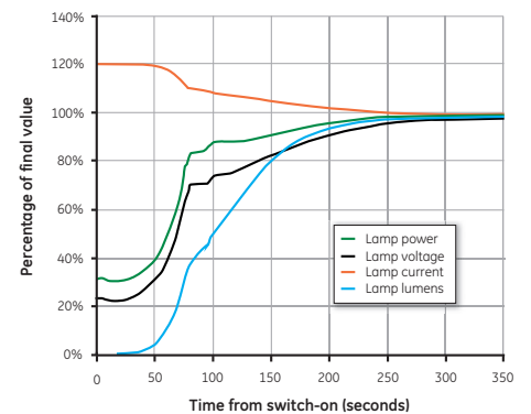
Typical warm-up characteristics for CMH TD 150W
