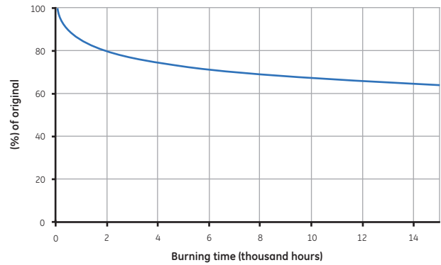
Lumen Maintenance for CMH70/TD
