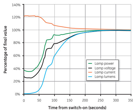
Typical warm-up characteristics for CMH TD 70W
