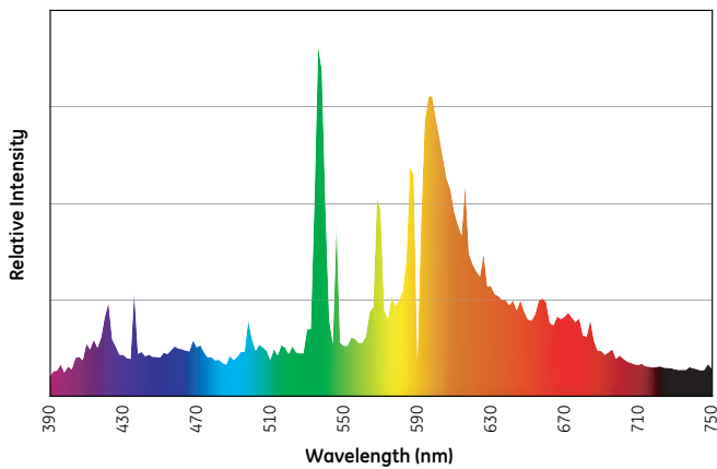
Spectral Power Distribution 3000K
