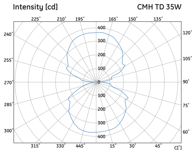
Horizontal plane polar intensity curve
