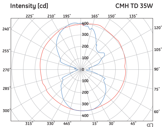
Vertical plane polar intensity curve
