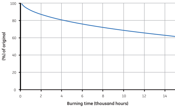
Lumen Maintenance for 150/TD
