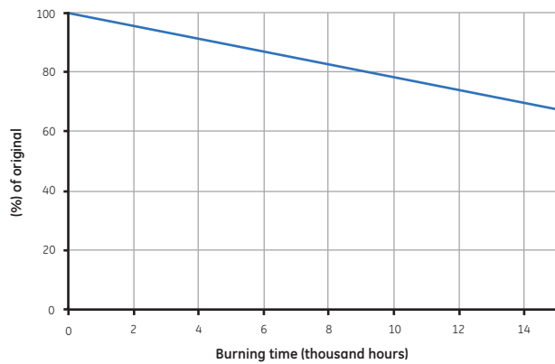
Lumen Maintenance for 150/TD
