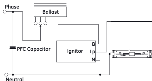
Typical superimposed ignitor circuit
