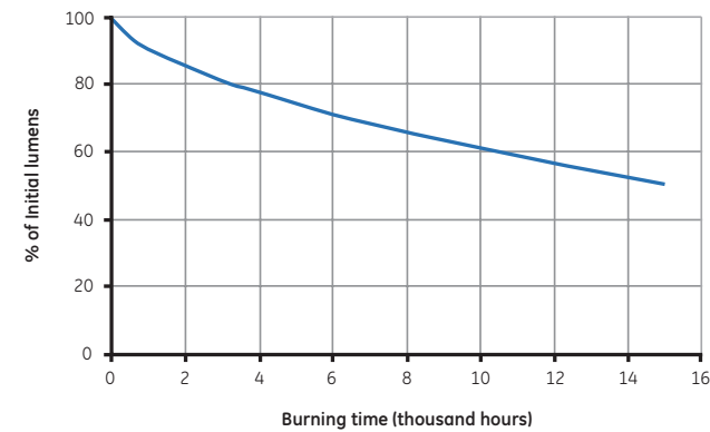
Lumen maintenance CMH G8.5 70W 3000K
