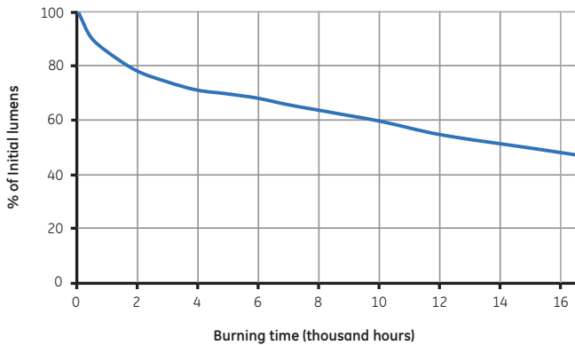
Lumen maintenance CMH G8.5 20W 3000K
